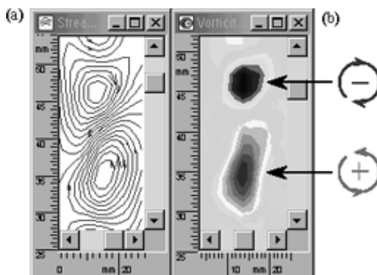
Figure 4. Streamlines (a) and vorticity (b) of flow field in the rotary tubular membrane separator with Re_a = 203.9 , Re_r = 2.745 and Ta = 6074 .
